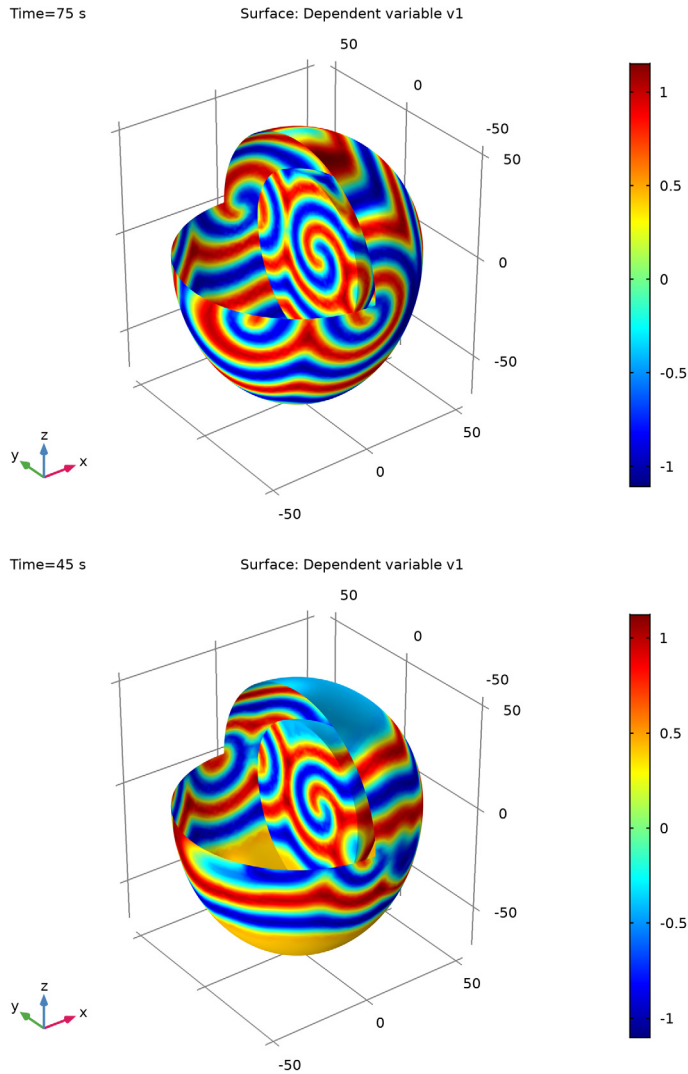
Figure 3: Solution to the Complex Landau-Ginzburg equations at times t = 75 s (top) and t = 45 s (bottom).
